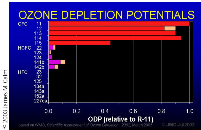
FIGURE 1. Ozone depletion potentials (ODPs) of common CFC, HCFC, and HFC refrigerants (based on WMO, "Scientific Assessment of Ozone Depletion: 2002," March 2003).
