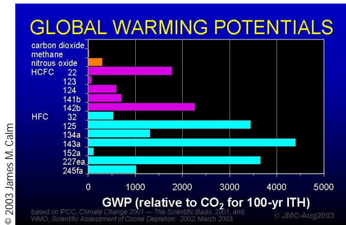
FIGURE 2. Global warming potentials (GWPs) of common HCFC and HFC refrigerants (based on IPCC, "Climate Change 2001 — The Scientific Basis," 2001, and WMO, "Scientific Assessment of Ozone Depletion: 2002," March 2003).
