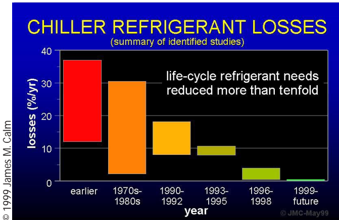
FIGURE 3. Progress in reducing refrigerant emissions from leakage, purge venting, and other operating and service losses.
