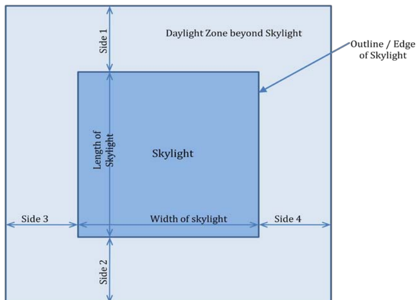
Plan View of Skylight and Daylight Zone
